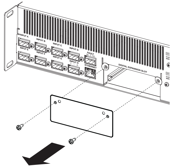
Figure 1. Remove cover plate from rear expansion slot
