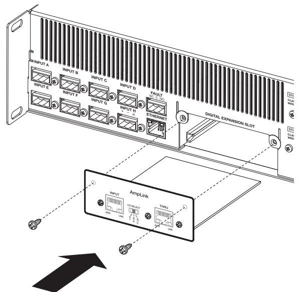
Figure 2. Insert AmpLink card into amplifier
