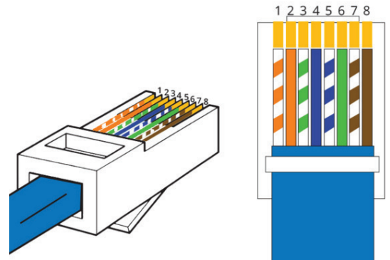
RJ45 Wiring - T568B
