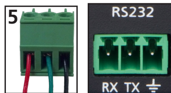
Pin out color will differ per RS-232 cable.
